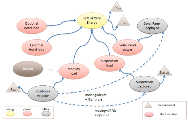
Figure 2. Energy state effects diagram
