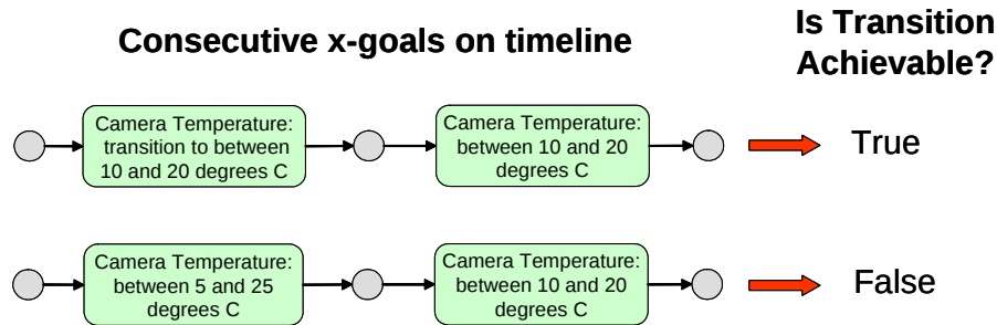
Figure 20. Transition achievability function.
