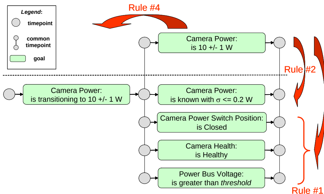
Figure 13. The elaboration for the “Camera Power State is 10 \pm 1 Watts” goal.
