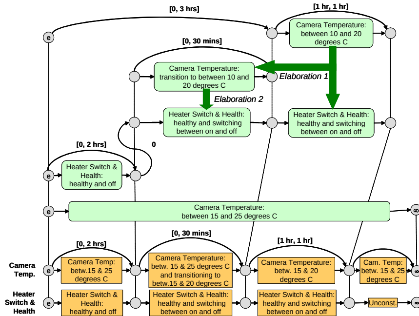
Figure 21. Scheduling example (top, before scheduling; bottom, after scheduling).
