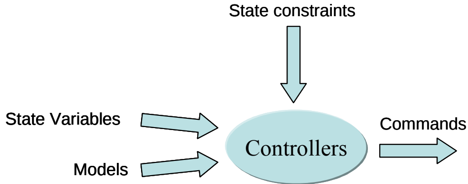
Figure 24. Controllers use state information, along with models of the system under control, to satisfy state constraints (goals) by issuing commands to the hardware adapters.
