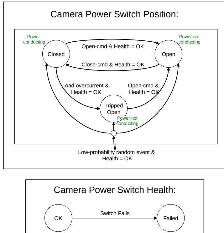
Figure 7. StateCharts for the Camera Power Switch Position and Camera Power Switch Health state variables. The three discrete state values for Camera Power Switch Position each have an associated power conduction behavior. This model allows for a low-probability random event that can change the switch position state arbitrarily, presuming the switch health is not Failed (i.e., stuck). This type of a single-event upset behavior, although rare, should be captured as a possible response of the switch.
