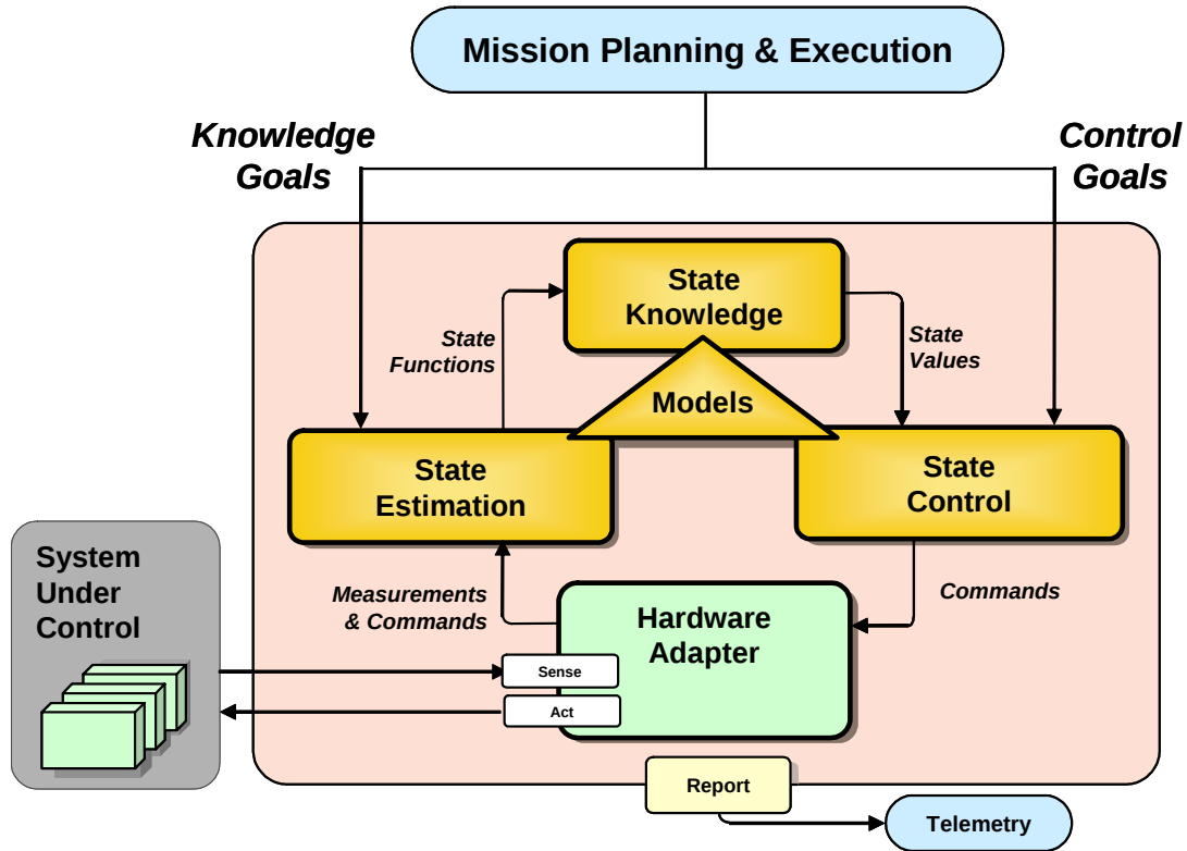
Figure 2. The state-based control architecture.
