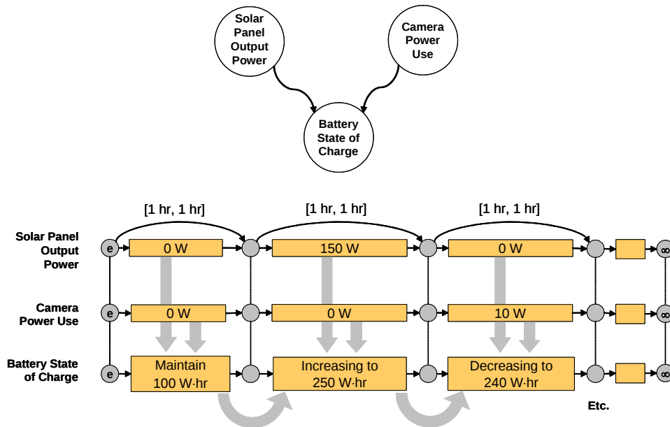
Figure 19. Projecting state effects across state over time. This simple example assumes that the Camera is the sole power user. The time point labeled “e” corresponds to an “epoch” reference time, and the time point labeled “∞” corresponds to infinity, denoting the end time point of the network. Though the temporal constraints on these x-goals are fixed 1-hour intervals, flexible temporal constraints are also supported.
