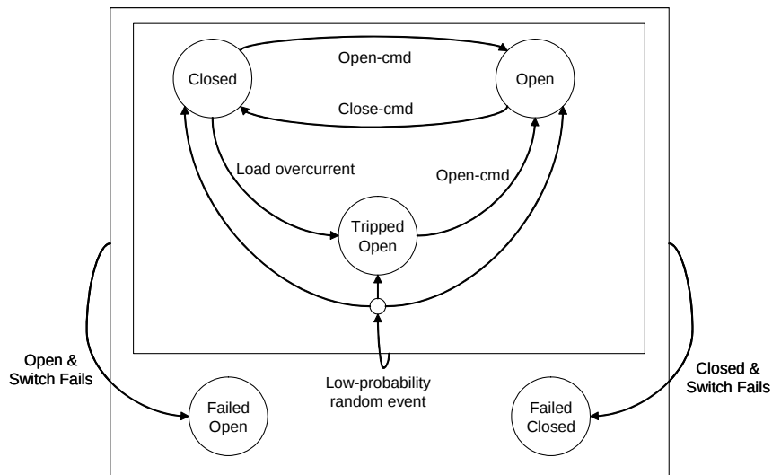
Figure 9. State model for the combined Camera Power Switch Position & Health state variable (StateChart representation).
