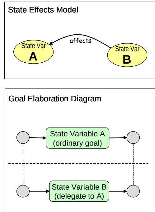
Figure 15. Reactive execution-time coordination via delegation is enabled during goal elaboration.
