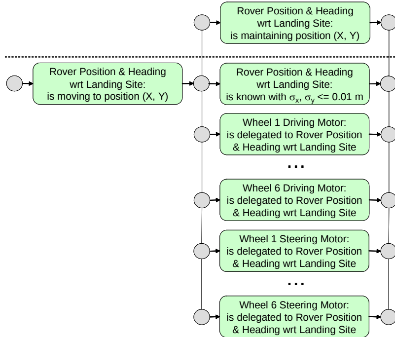
Figure 16. Goal elaboration that establishes delegation of wheel motors for driving and steering to Rover Position & Heading controller.
