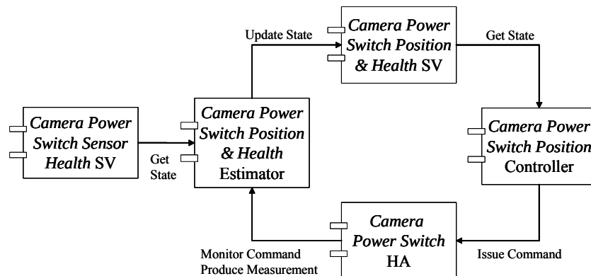
Figure 26. Collaboration diagram showing the estimation and control pattern for the Camera Power Switch Position and Health state variable.
