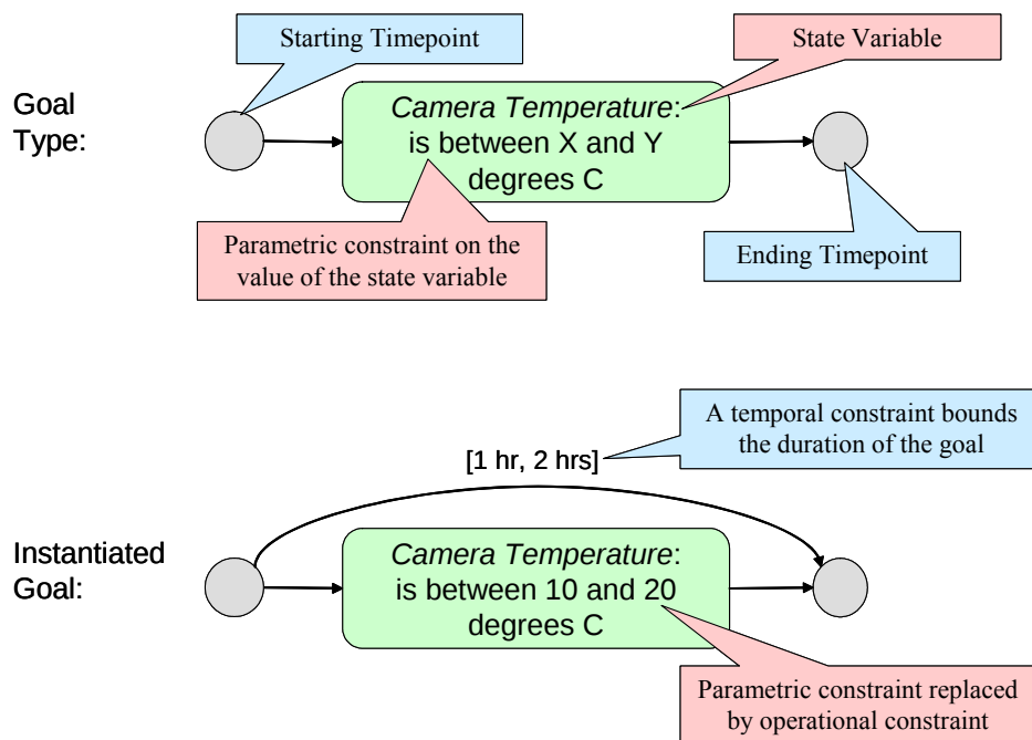
Figure 12. The anatomy of a goal type and an instantiated goal. Every goal has a starting time point and an ending time point. A goal can be instantiated with a flexible temporal constraint on its duration, indicated by an arrow from its starting to its ending time point, labeled with a [min, max] duration window.
