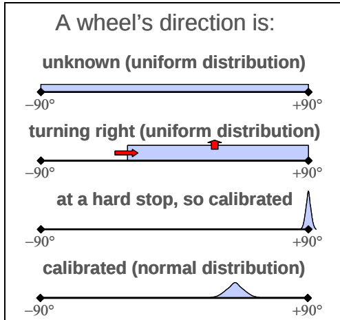
Figure 4. Uncertainty representation can be polymorphic, e.g., given a uniformly uncertain rover wheel direction, we can calibrate our knowledge of direction by turning the wheel (narrowing the range of the uniform distribution) until it hits its stop (at which point our knowledge of state has very little uncertainty). As a result of rover operations, the level of uncertainty in the wheel direction estimate increases over time (represented as a normal distribution with gradually increasing variance).
