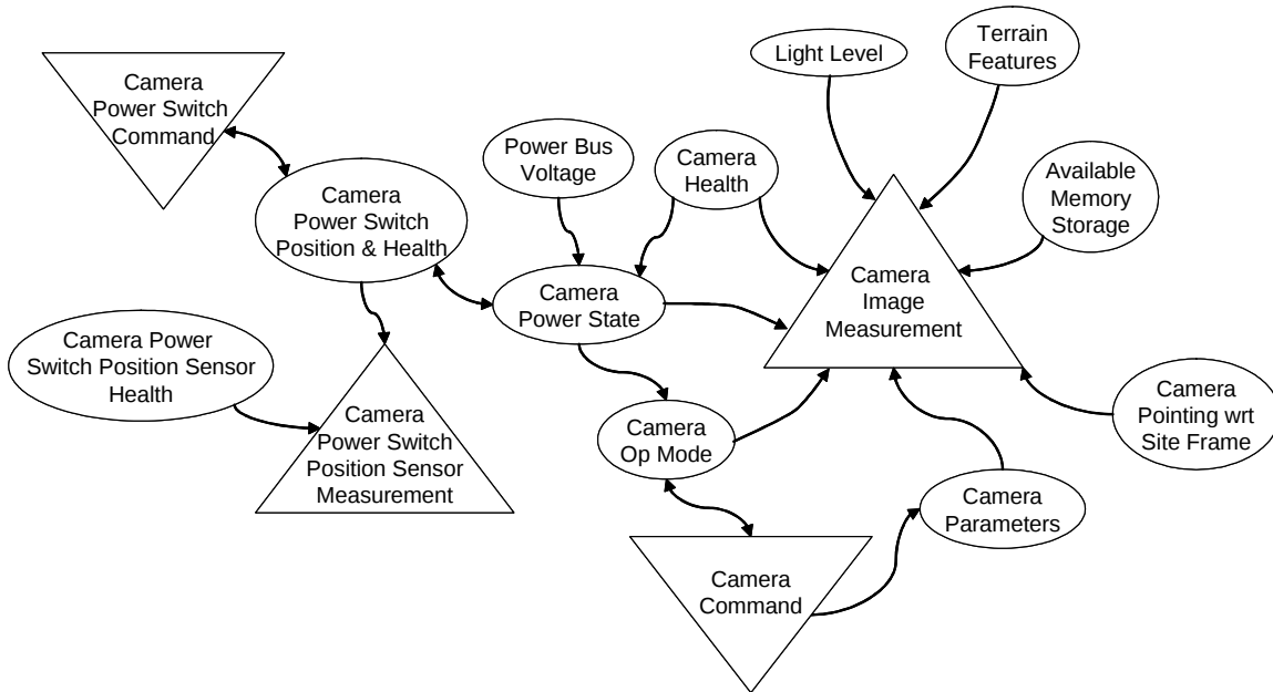
Figure 11. State Effects Diagram for simple camera example.
