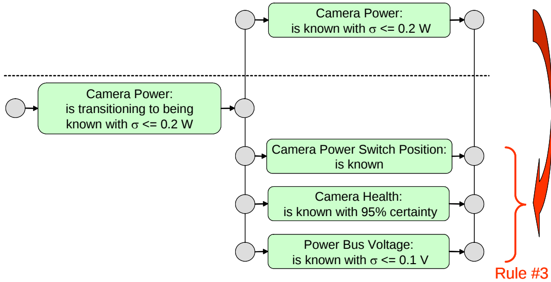
Figure 14. The elaboration for the “Camera Power State is known with \sigma \leq 0.2 Watt” goal.
