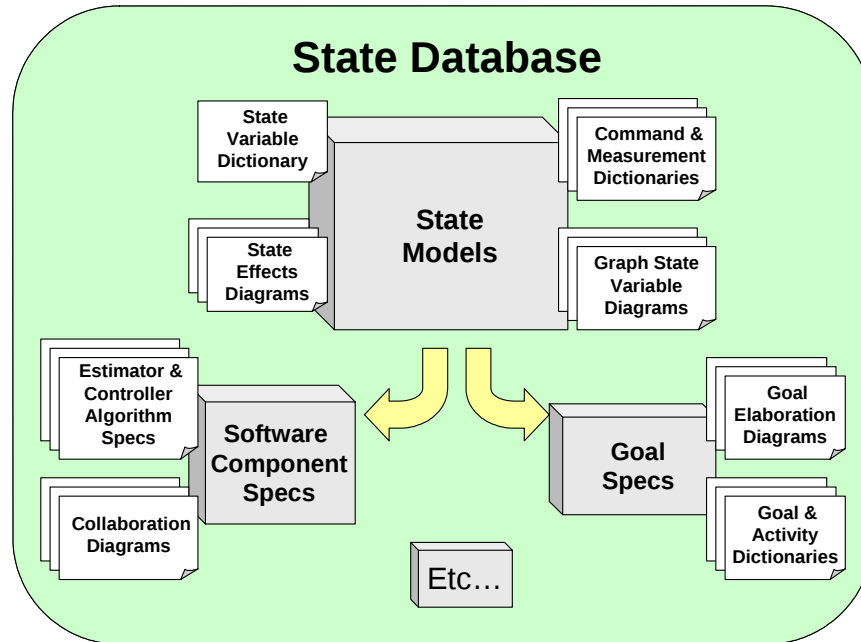
Figure 27. State Analysis products captured in the State Database.
