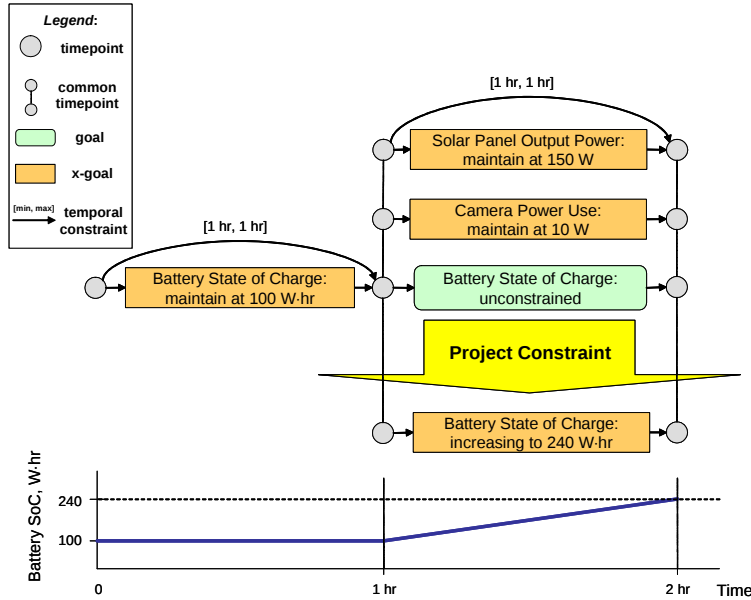
Figure 18. Projecting effects across the state variables of the system under control. Lower plot depicts the resulting constraint on Battery State of Charge vs. time.
