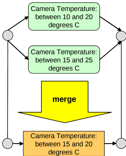
Figure 17. Goal merging function.
