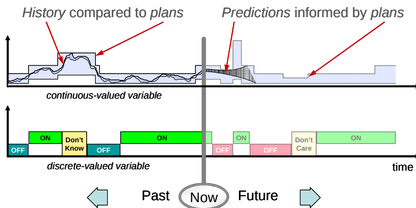
Figure 3. Timelines are used to capture state knowledge (past estimates and future predictions) and intent (past and future constraints on state).
