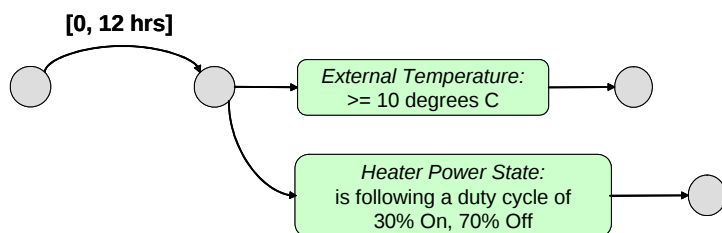
Figure 22. Goal network that illustrates event-driven execution using a goal on an uncontrollable state variable.
