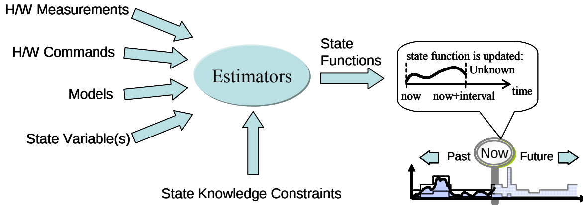
Figure 23. Estimators use measurement, command and state information, along with models of the system under control, to satisfy state knowledge constraints (goals) by updating state in the form of state functions.
