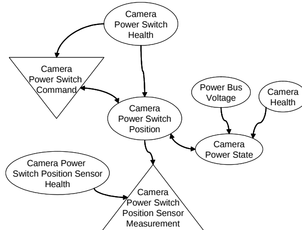
Figure 8. State Effects Diagram after two iterations of the modeling process.
