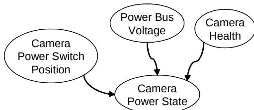
Figure 6. State Effects Diagram after one iteration of the modeling process. State variables of the system under control are represented as ovals, and state effects are denoted by arrows.
