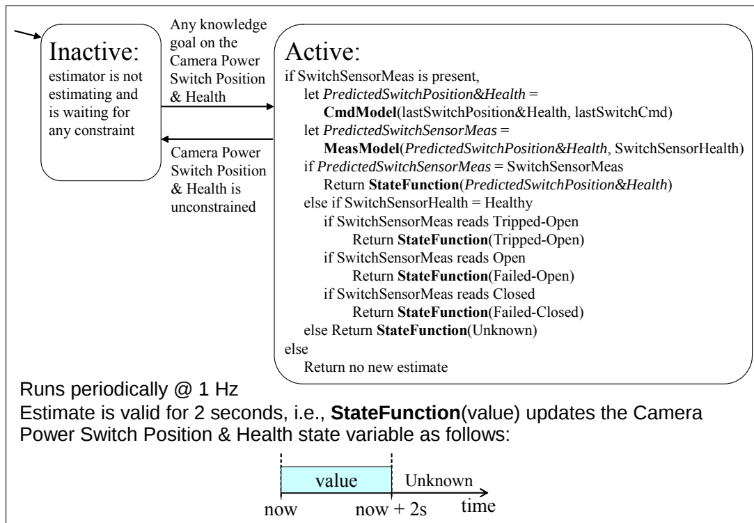
Figure 25. Simple estimator for Camera Power Switch Position & Health. It uses the Camera Power Switch Sensor Measurement Model and Camera Power Switch Command Model, and it updates the Power Switch Position & Health state variable using a State Function. [SV: state variable; HA: hardware adapter]
