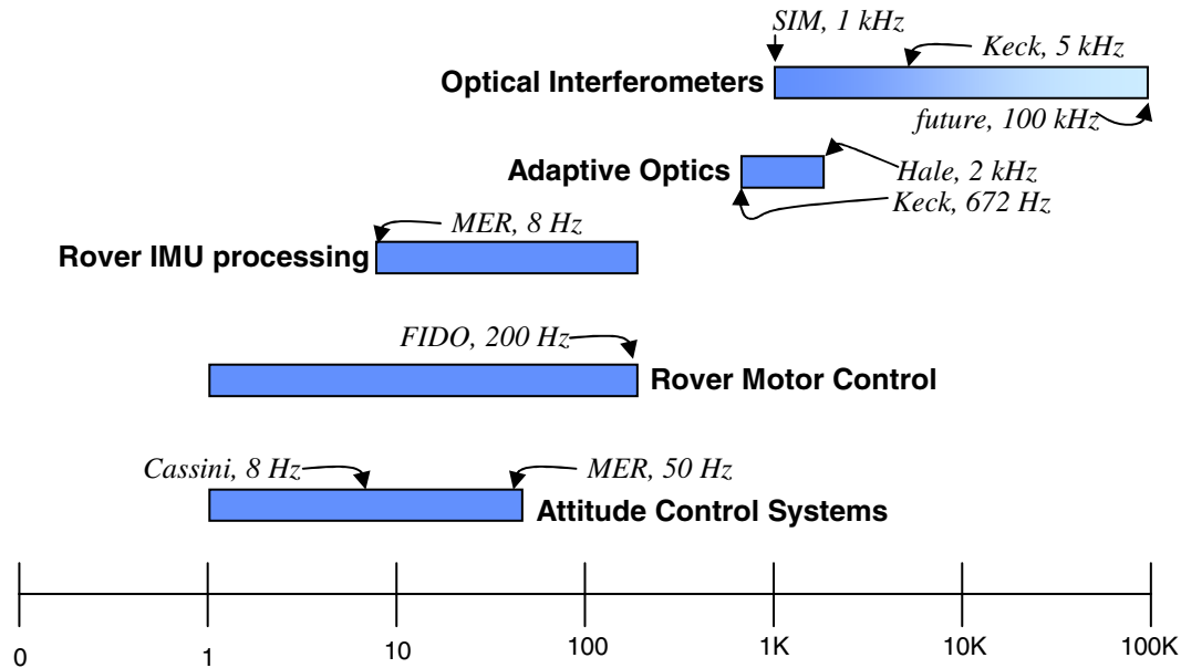
Figure 1. Software control loop frequency in Hz
