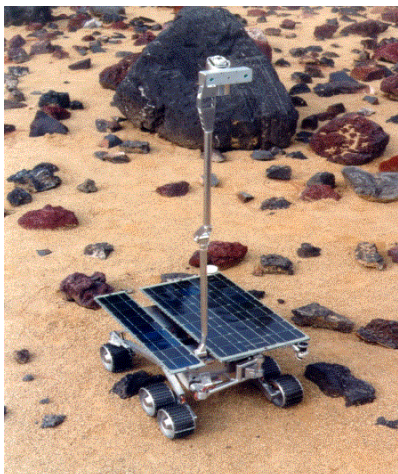
Figure 2. Rocky 7 rover at work in the JPL Mars Yard.
